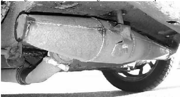
XP-exhaust system with the long reverse cone
